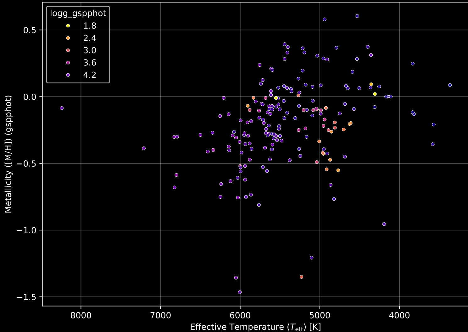
APOGEE DR17 Field: [140+62_MGA] Stellar Population Parameters (n= 187)
