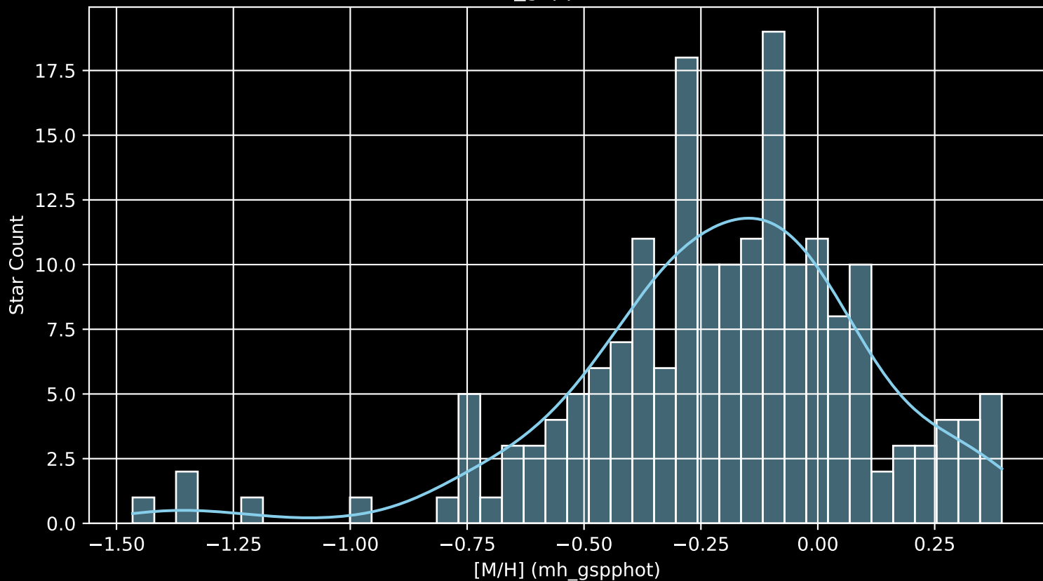
APOGEE DR17 Field: [140+62_MGA [M/H] (mh_gspphot) (n= 185)
