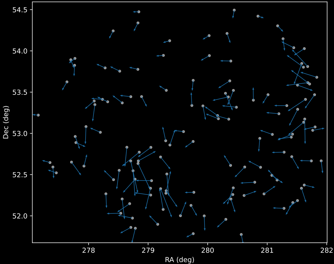
APOGEE DR17 Cluster 0 Proper Motion Vectors (n=131)
