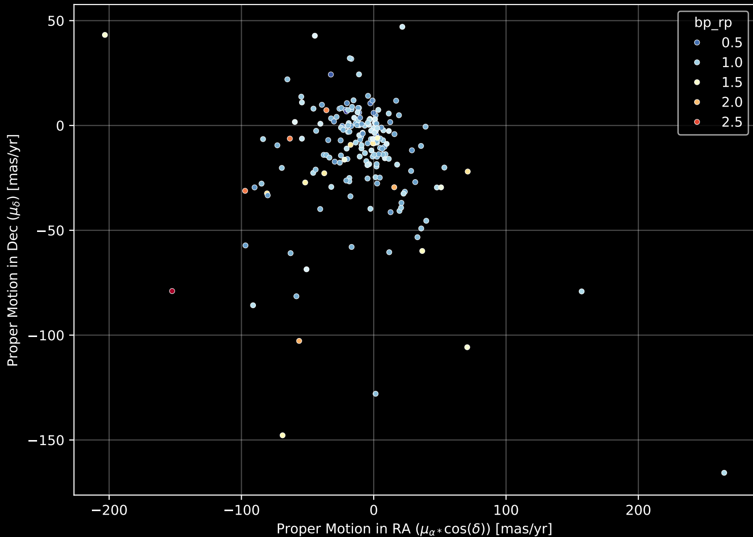
APOGEE DR17 Field: [140+62_MGA] Proper Motion Diagram (n= 187)
