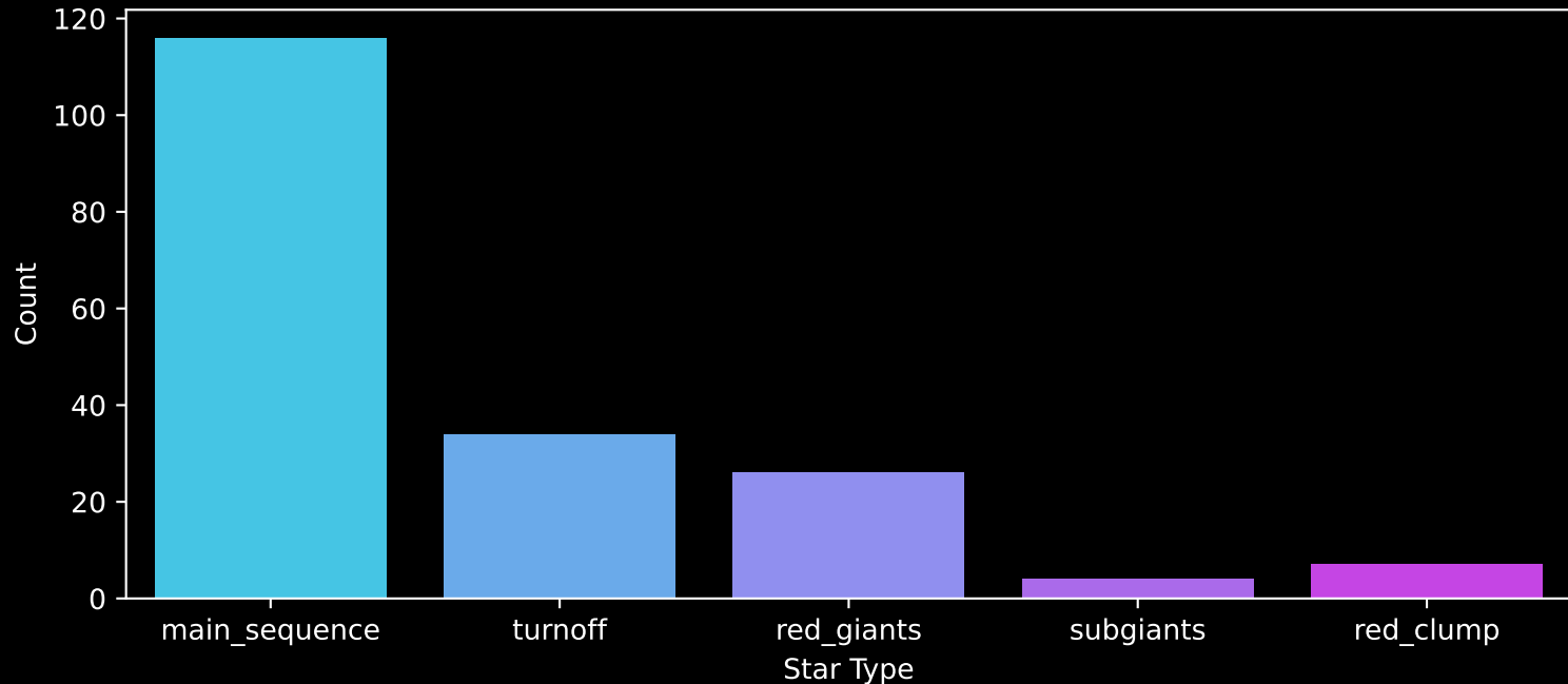
APOGEE DR17 Field: [140+62_MGA] Count plot of Star Type
