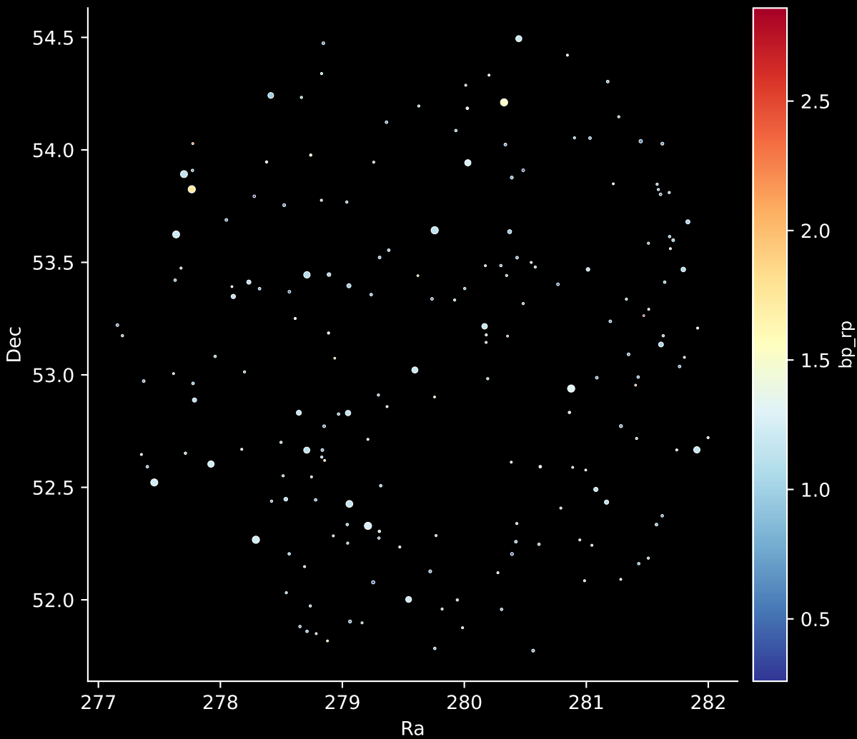
APOGEE DR17 Field: [140+62_MGA] Stars: 187
