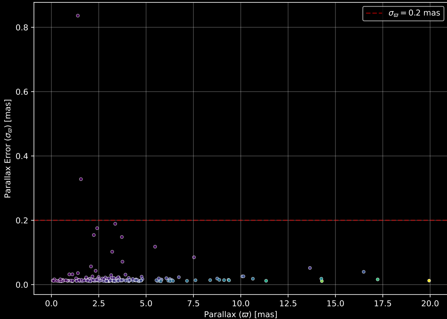
APOGEE DR17 Field: [140+62_MGA] Parallax Quality (n= 187)
