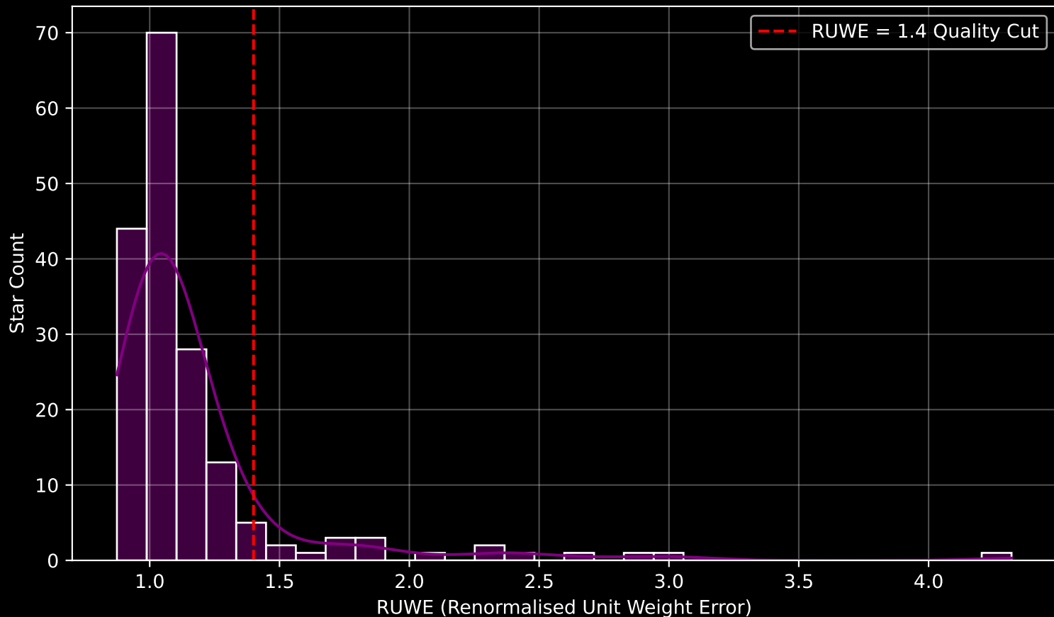
GAPOGEE DR17 Field [140+62_MGA] RUWE Distribution (n= 177)
